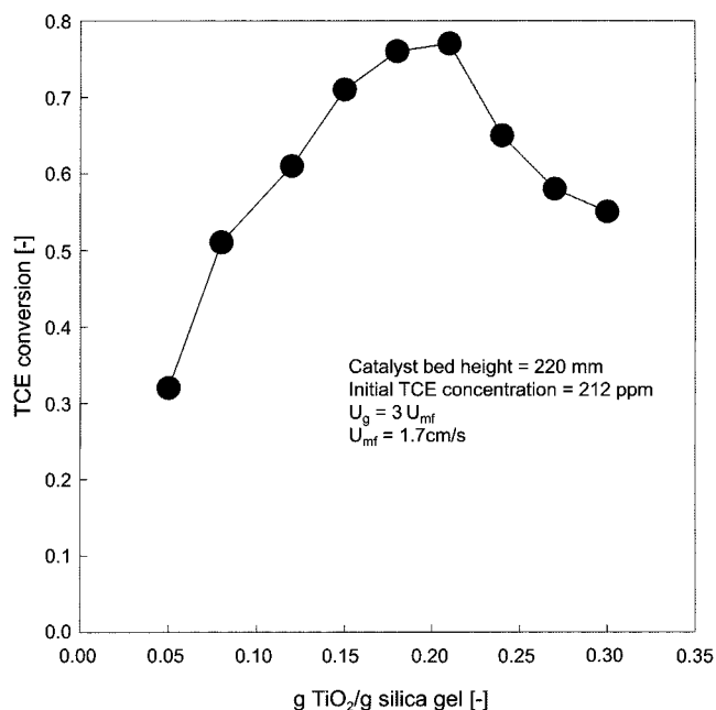
Fig. 3. Effect of \text{TiO}_2/\text{silica gel} ratio on TCE conversion.
